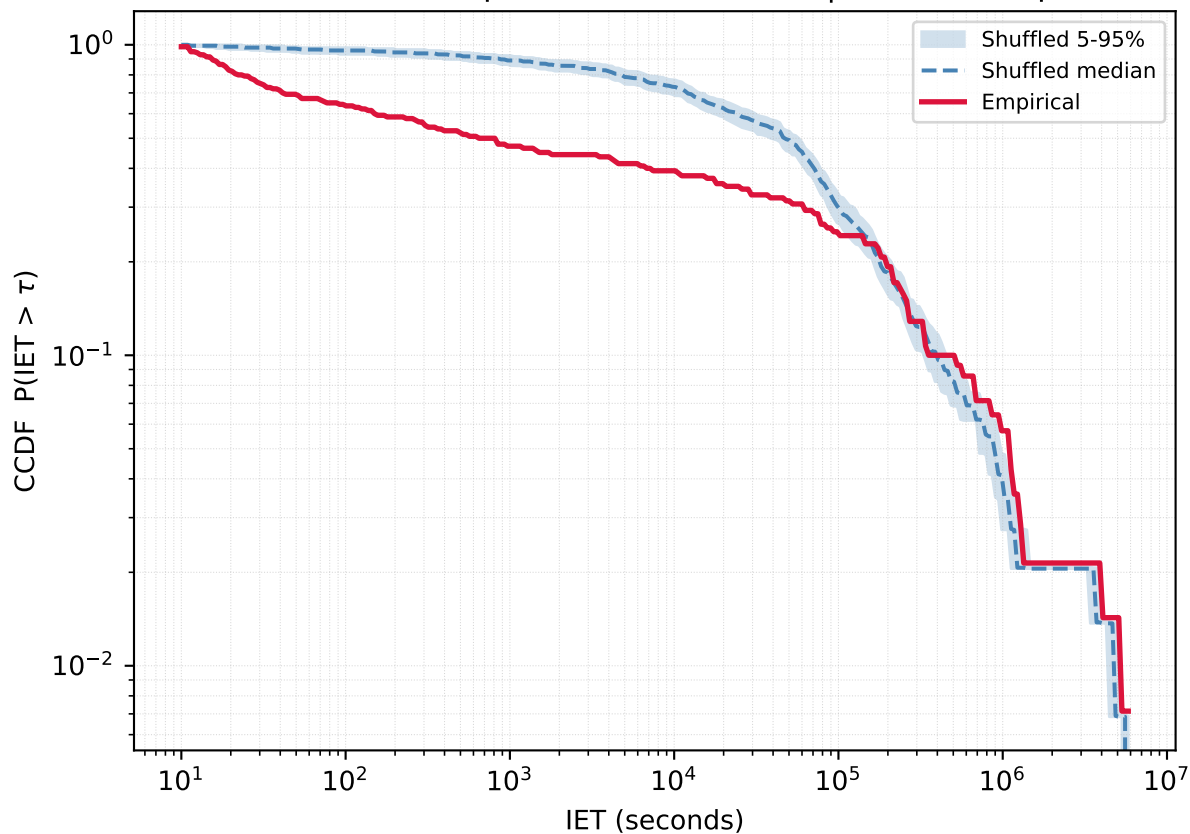
User 323309626 - Empirical vs Reshuffled | KS=0.430 p=0.000
